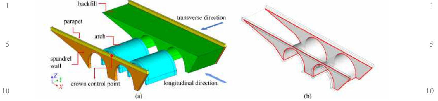
Fig. 4 (a) Different components of the numerical model of the Roman bridge and loading directions in addition to the location of control (crown) point; (b) CIE used to model the bridge.
