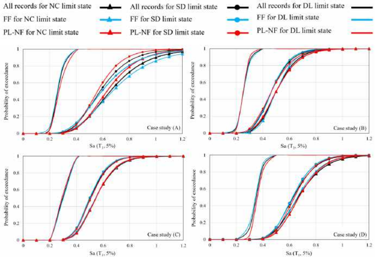
Figure 11: Fragility curves of the case studies subjected to FF and NF ground motions for all three damage limit states.
