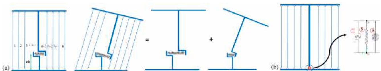
Fig. 7. (a) Kinematics of the conventional MVLEM element subjected to lateral and axial (compression) loadings, and (b). the modified MVLEM element for developing the macroelement to nonlinear modeling of URM buildings.
