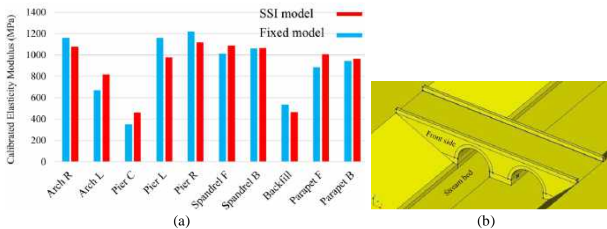
Figure 9: (a) Updated E values of different parts of the SSI and fixed-base models (b) stream bed location and front side of the bridge model.
