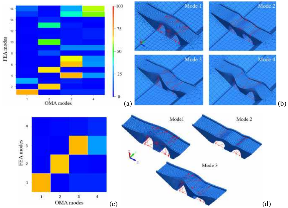
Figure 8: (a) MAC matrix and (b) mode shape correlations of the SSI model, (c) MAC matrix, and (d) mode shape correlations of the fixed-base model.
