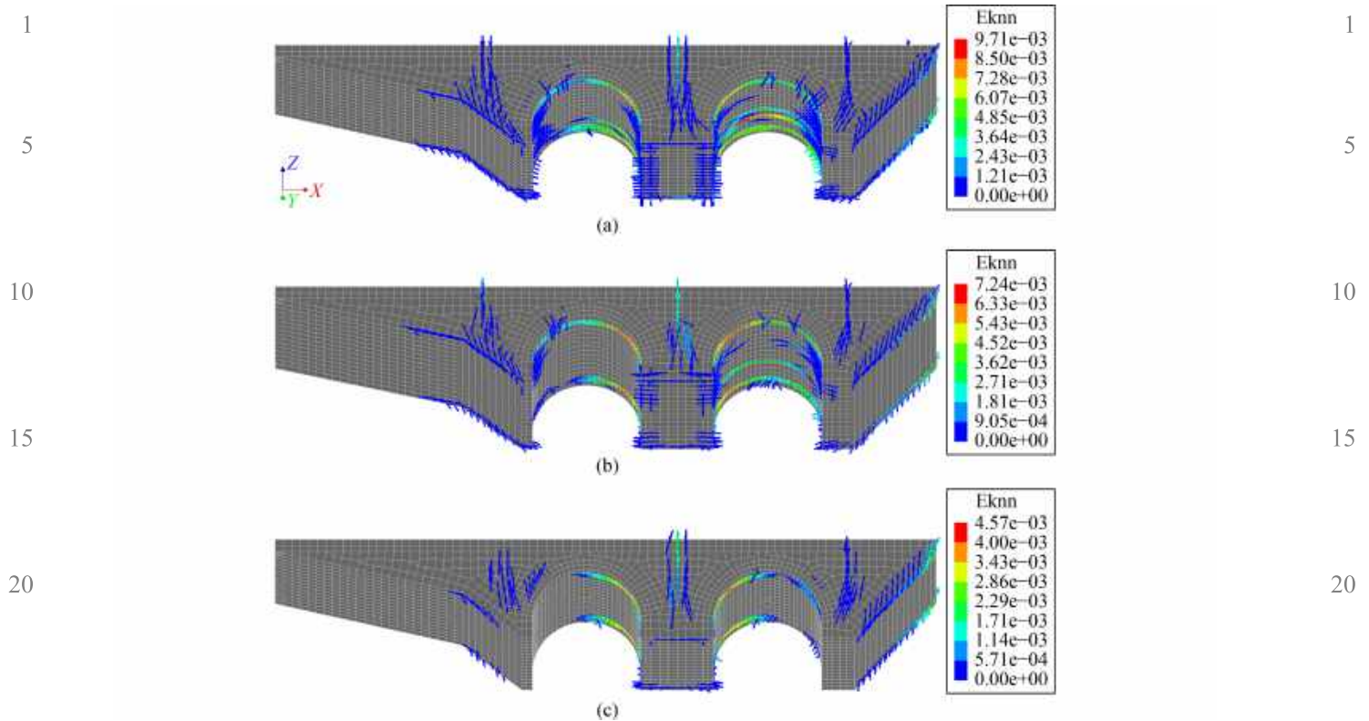
Fig. 17 Crack pattern and principal crack strain values for: (a) RSN 1083 ; (b) RSN 1013 ; (c) RSN 126 .
