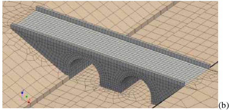
Figure 5: (a) 3D mesh of the SSI model (b) mesh details of the bridge.
