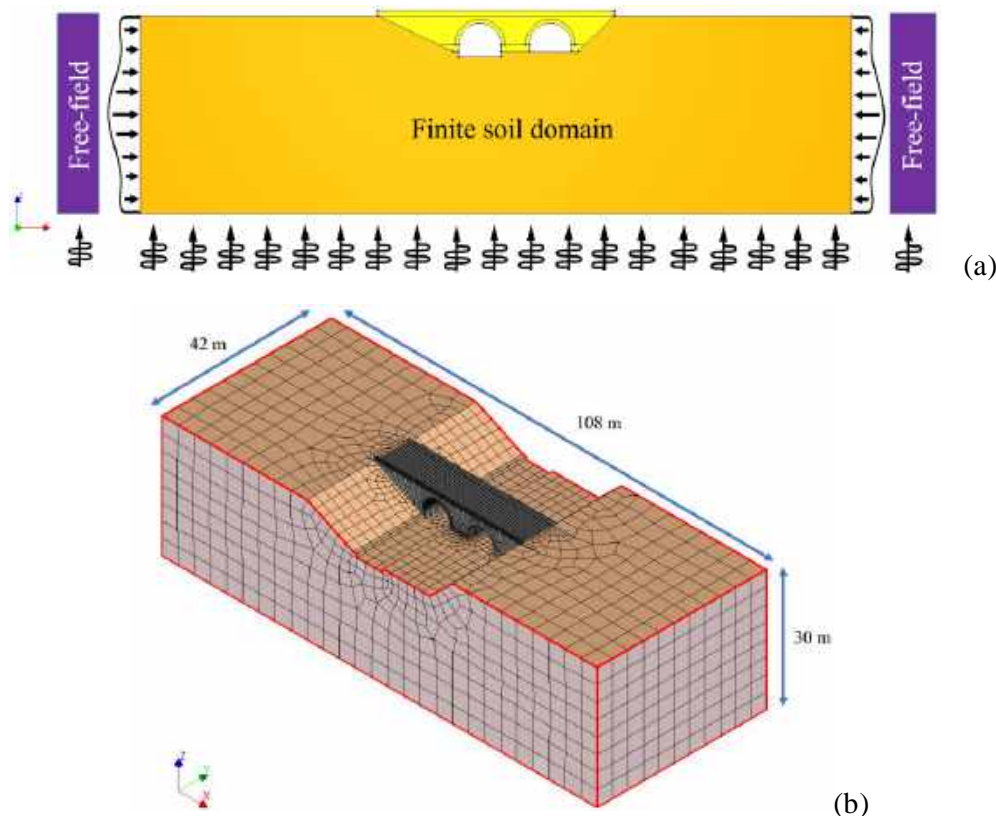
Figure 11: (a) Schematic representation of the free-field elements and (b) dimension of the SSI model with free-field boundary elements.
