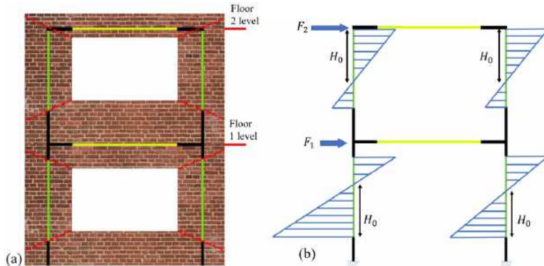
Figure 4: (a) A perforated two-story URM wall, and (b) moment diagram of the wall subjected to lateral loadings and definition of H_0 .
