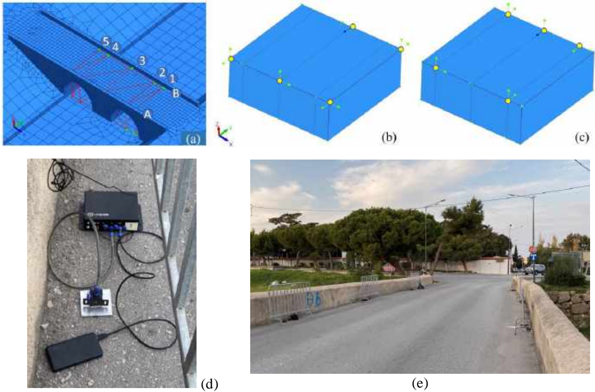
Figure 6: (a) Optimal sensor locations and sensors' configuration of the (b) first and (c) second test setups. (d) From top to bottom: datalogger, accelerometer sensor, and power bank, and (e) AVT campaign of the Roman Bridge.
