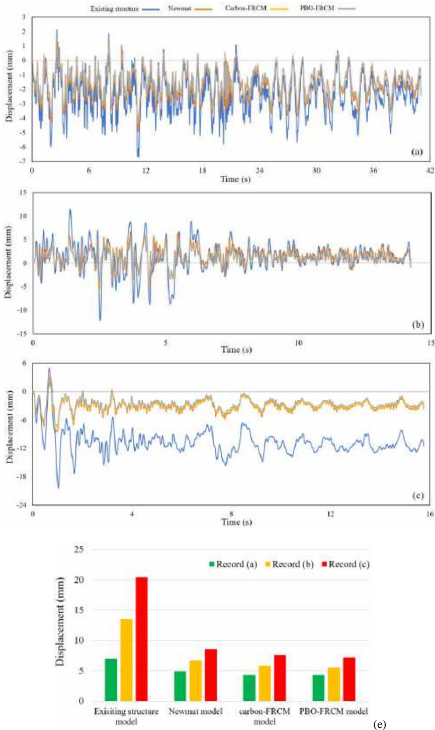
Figure 18: Displacement time history response of the crown nodes of the SSI and strengthened models subjected to record (a), (b), (c), and (e) maximum displacement values.
