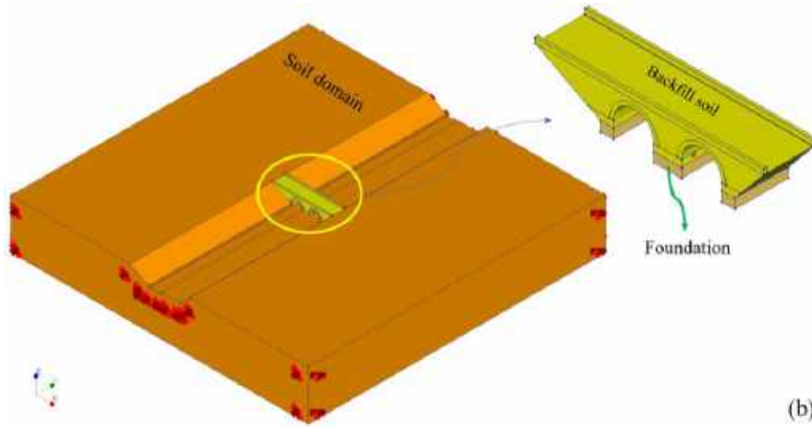
Figure 4: (a) Fixed-base 3D model, and (b) SSI model of Roman bridge.
