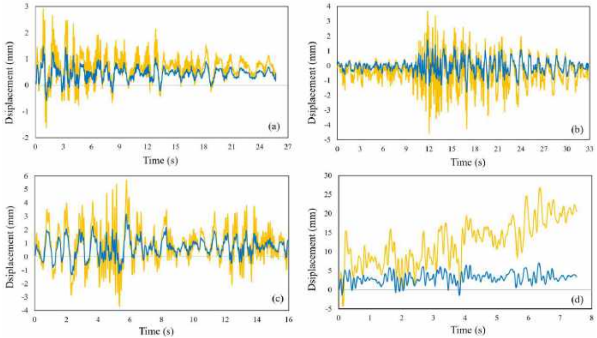
Figure 15: Displacement response time history of the crown nodes of the models subjected to the seismic records that impose (a) slight, (b) moderate, (c) extensive damages (d) complete collapse to the SSI model.
