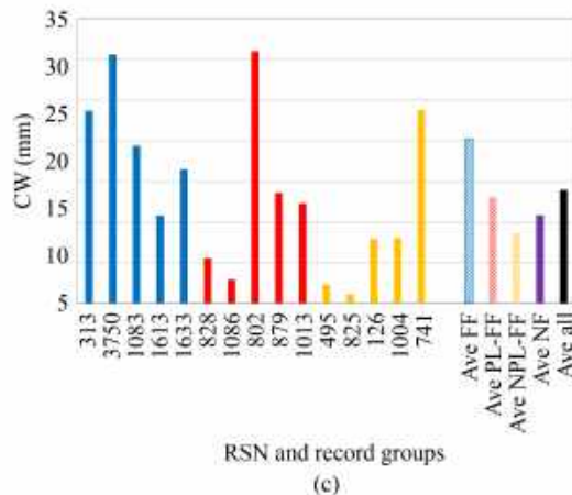
Fig. 13 Results of NLTHA in terms of: (a) maximum crown point displacement; (b) cracked volume damage index; (c) crack width.
