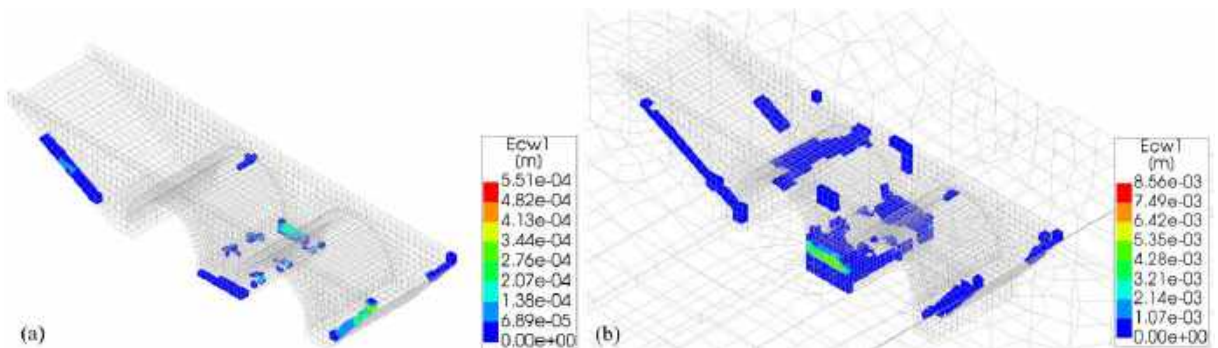
Figure 16: Crack pattern and width of (a) fixed-base and (b) SSI models subjected to the seismic records that impose extensive damages to the SSI model.
