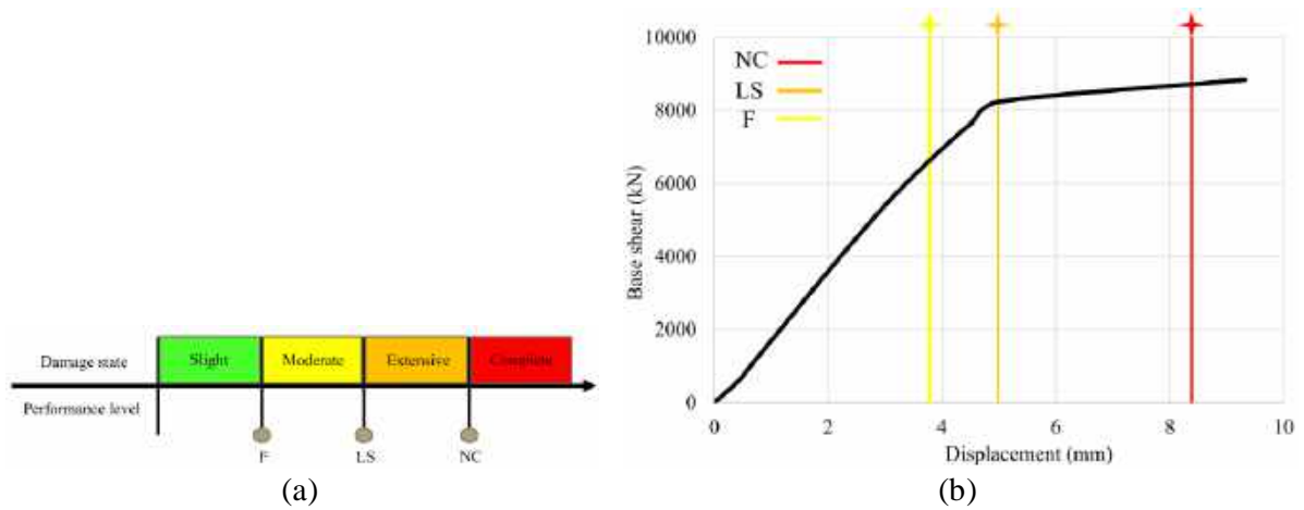
Figure 12: (a) Relationships between performance levels and damage states, (b) pushover curve and performance limits of the Roman bridge.
