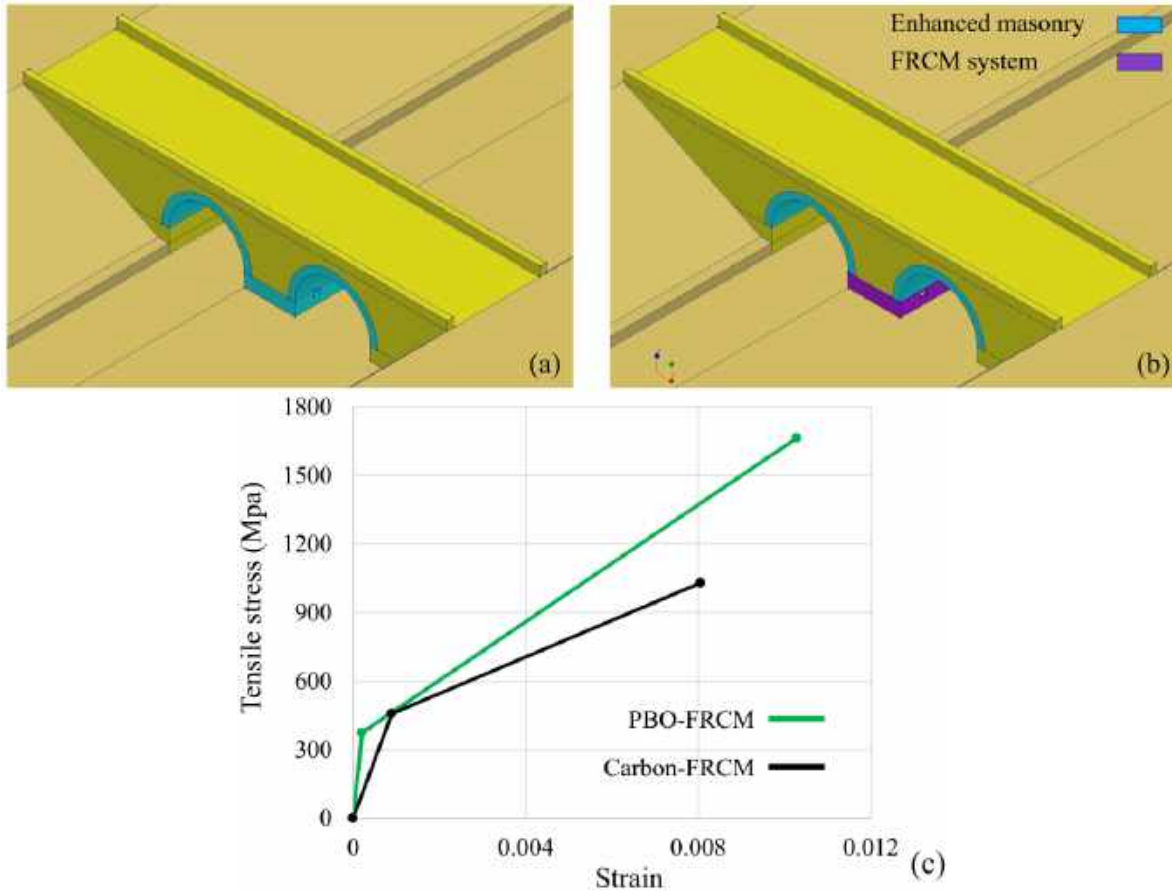
Figure 17: (a) Newmat and (b) FRCM strengthened models, and (c) stress-strain curve of FRCM systems in tension.
