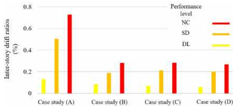
Figure 9: Determined limit states for the case studies from the pushover analysis
