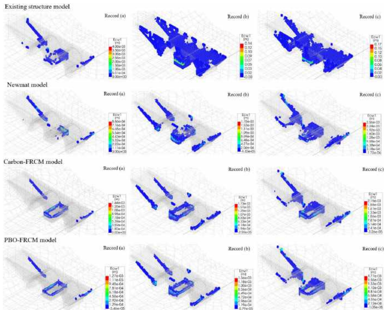
Figure 19: Crack patterns and width values of the existing structure model and strengthened models subjected to the three chosen seismic excitations.
