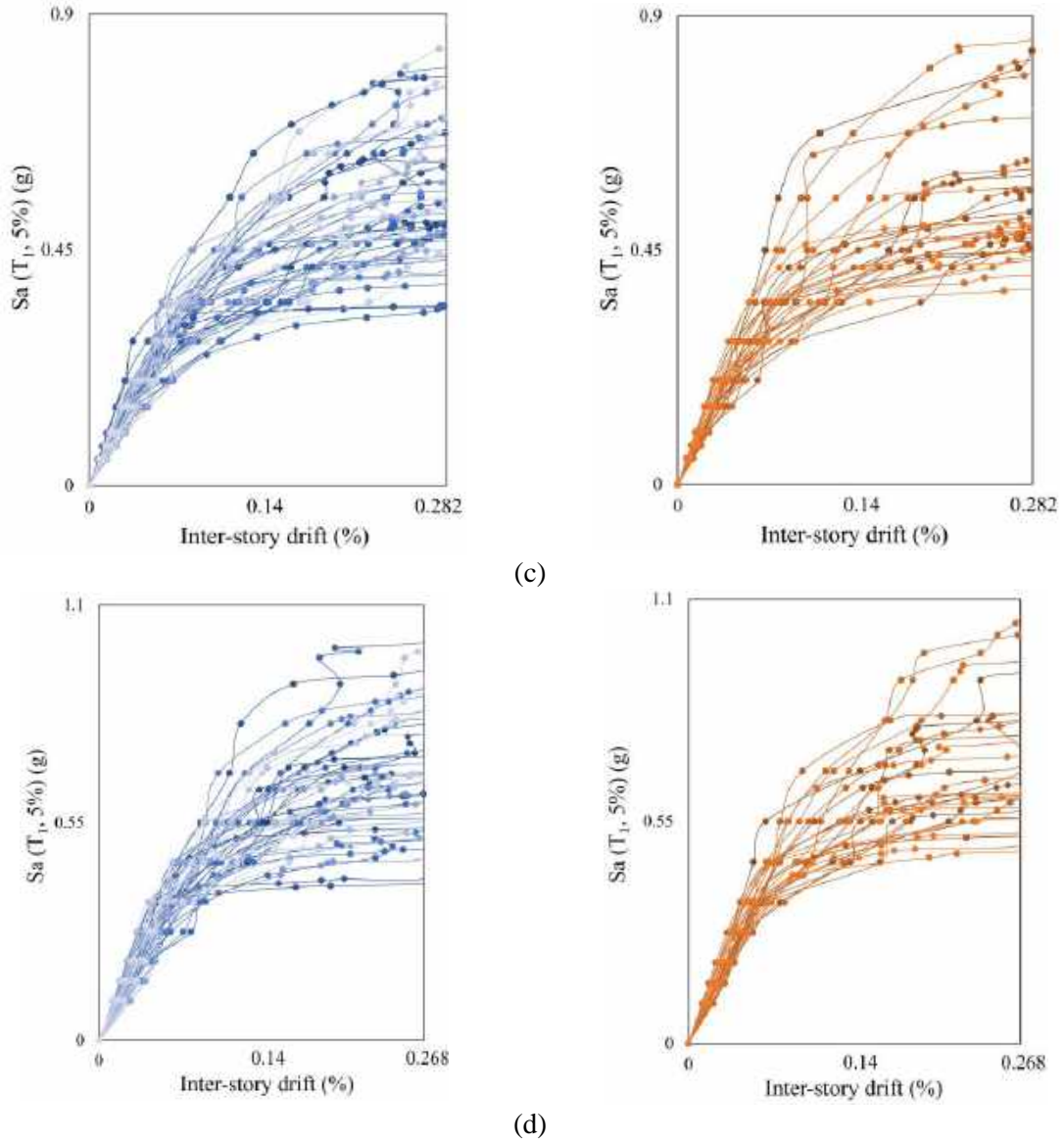
Figure 10: IDA curves of the case studies subjected to FF and NF ground motions.
