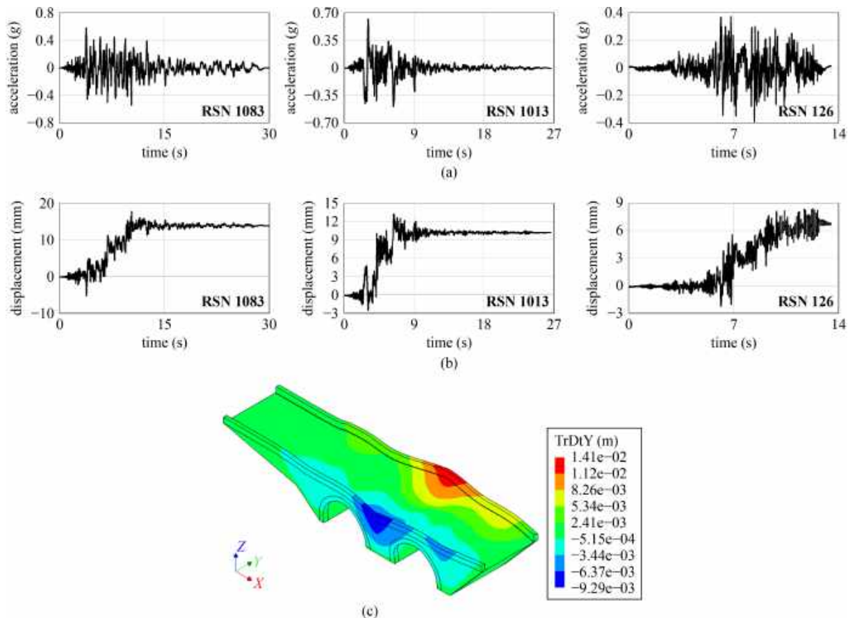
Fig. 16 (a) Accelerograms of RSN 1083 , RSN 1013 , and RSN 126 events; (b) displacement response time history of the crown points; (c) magnified deformed shape of the bridge subjected to RSN 1083 record at the end of the analysis.
