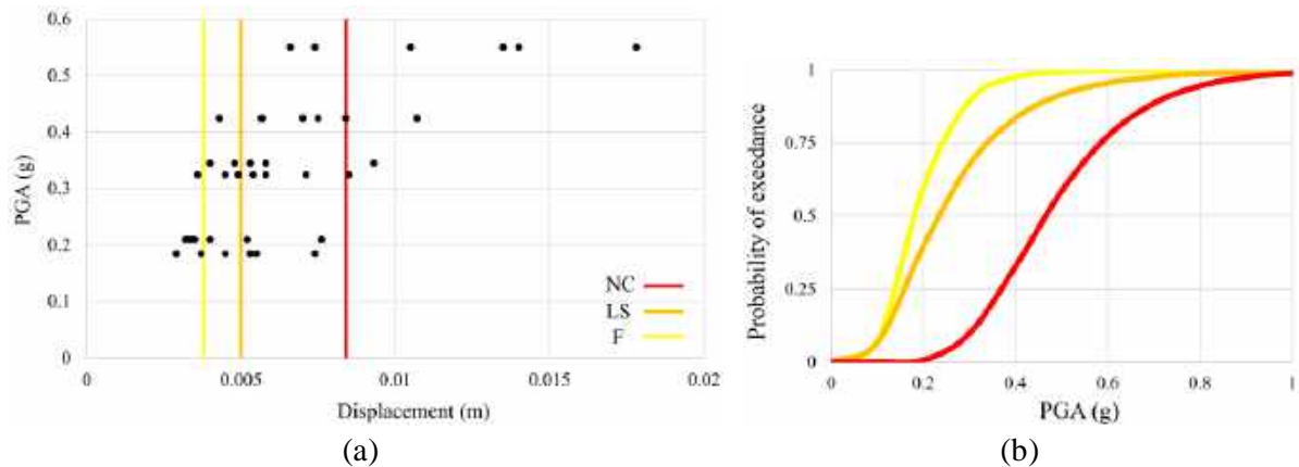
Figure 14: (a) MSA results with performance limit values, (b) seismic fragility curves of the case study.
