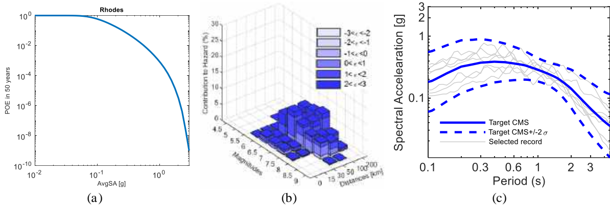
Figure 13: (a) Hazard curve for AvgSA, (b) Disaggregation of the hazard and (c) selected records based on the CS record selection approach for the 10% probability of exceedence in 50 years.
