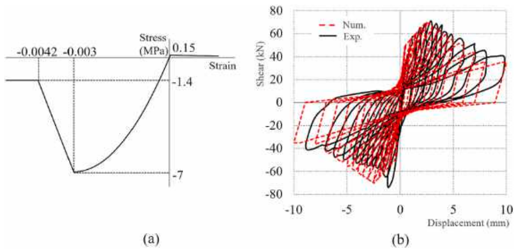
Fig. 14. (a) stress-strain curve of masonry based on the Concrete02 material, and (b) experimental-numerical comparison curves of the spandrel element.
