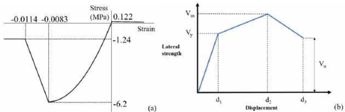
Figure 3: (a) Stress-strain curve of URM and (b) trilinear backbone curve of the nonlinear shear spring.
