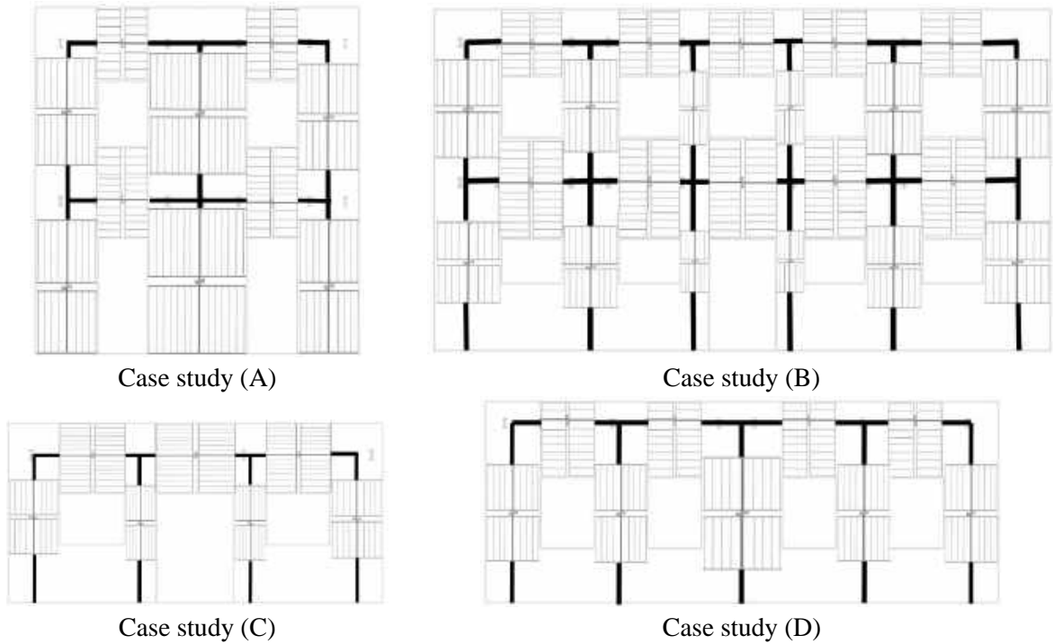
Figure 2: Developed nonlinear models of the four case studies using DM-MVLEM macroelement.
