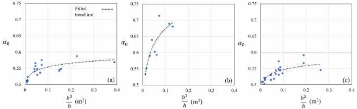
Figure 6: The results of the regression analysis and trendlines of the data derived from analysis of (a) internal piers of the first story, (b) external piers of the first story, and (c) piers of the second story.
