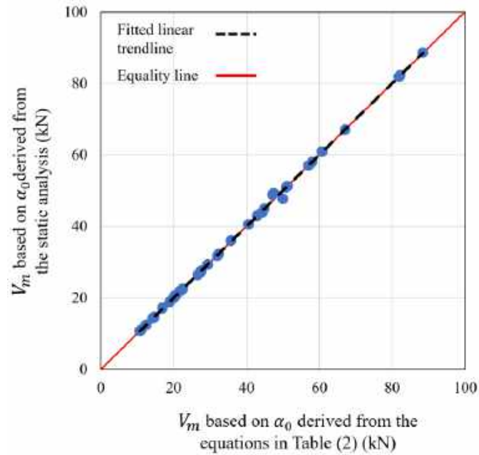
Figure 7: Scatter plot and equality line for the results of the V_m based on \alpha_0 derived from the static analysis and proposed equations.
