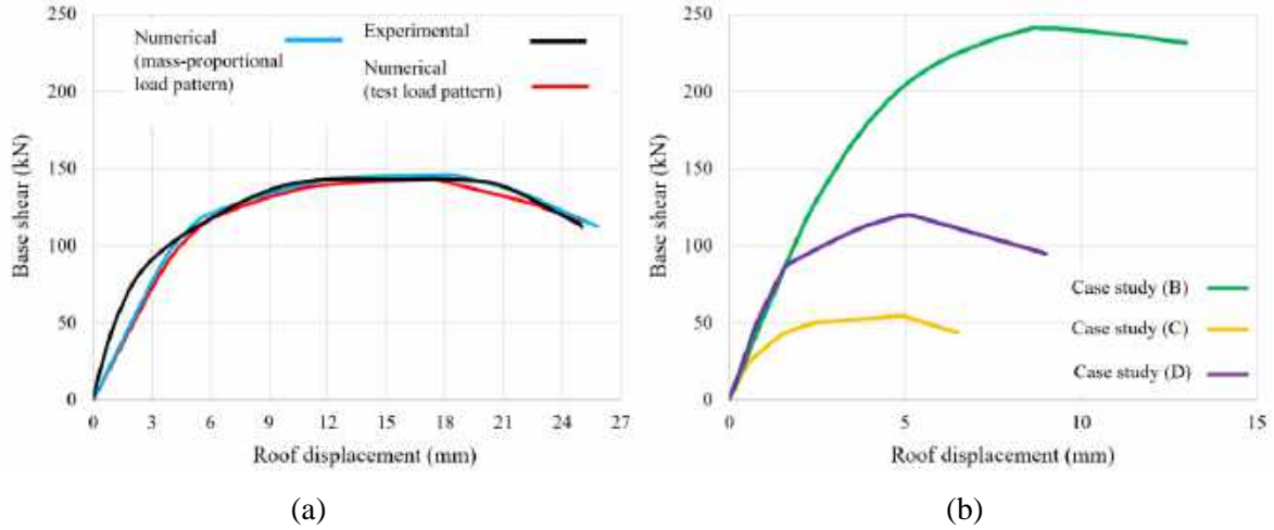
Figure 8: Pushover curves of (a) case study (A) (Pavia door wall) with the test results and (b) other case studies.
